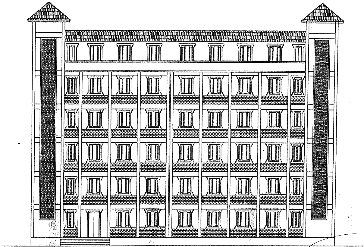
FRONT ELEVATION
